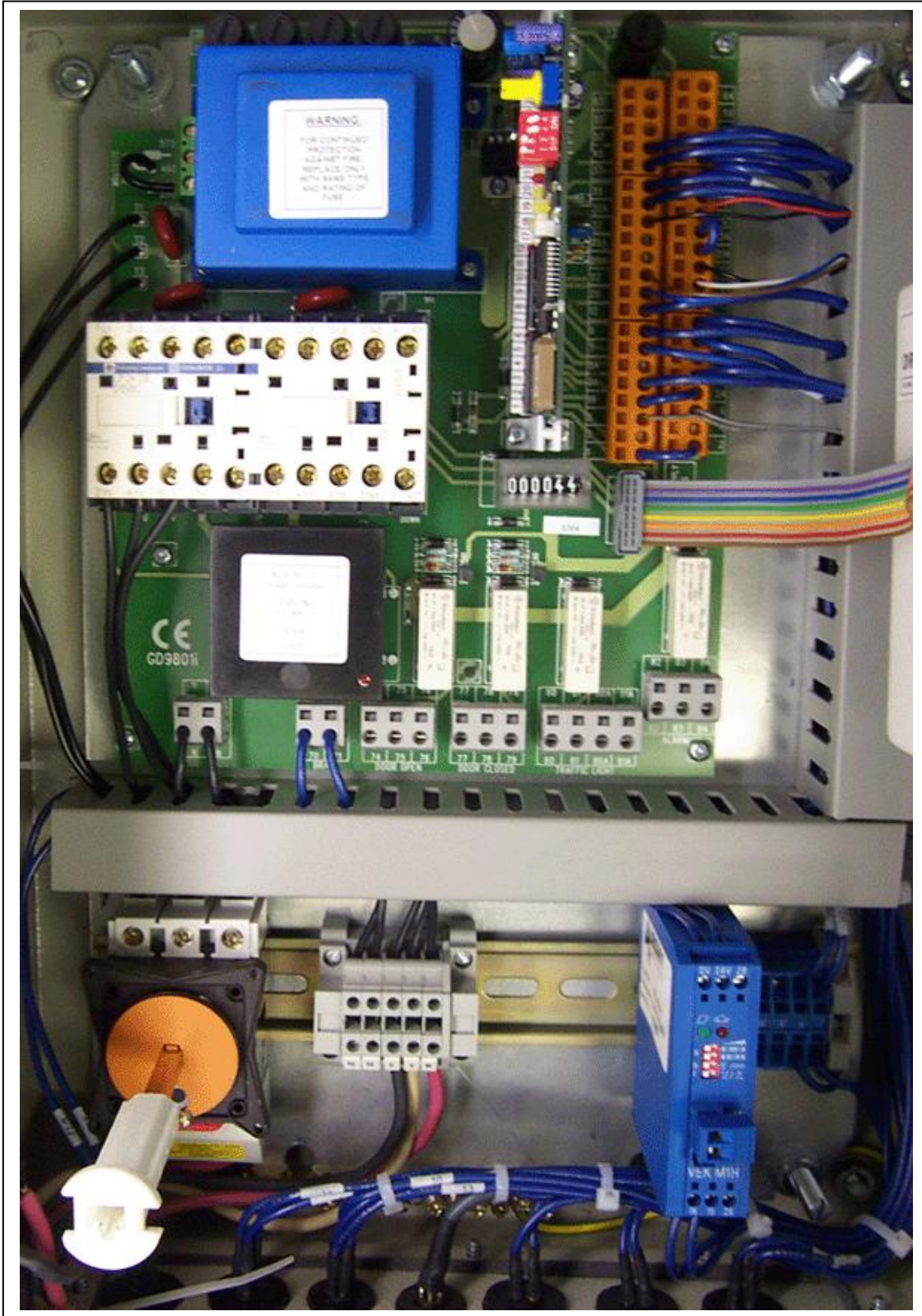
The ACS50 Control Panel Interior (Single speed)
